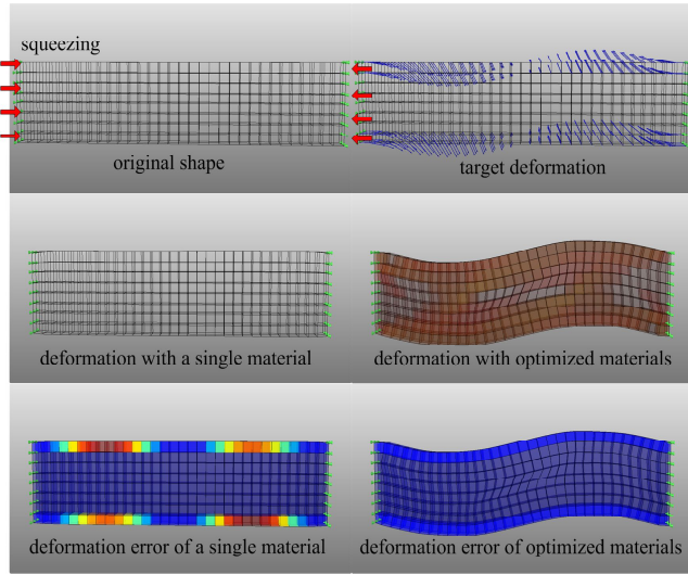
Fig. 10. Optimizing a beam to make it bend when it is squeezed. A beam with optimized material properties can take the desired shape (right) whereas a beam with homogeneous material properties can only axially deform under small deformation (left). In this example, the vertices on the vertical sides are fixed in their target positions, while the other vertices are free to move. Target displacements are set on the nodes of the cells of the two horizontal boundary layers. The color plot for the bottom beams shows the deformation error of each cell as defined by Equation 13.
