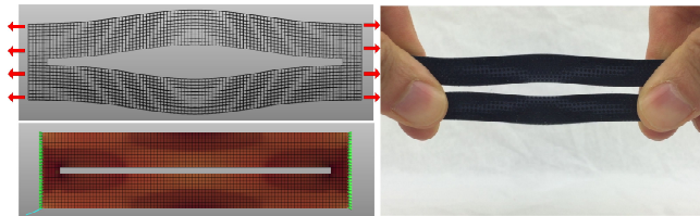
Fig. 19. An optimized hollow beam with target deformation. The left figure shows the target deformation and optimized material distribution. The right figure shows the 3D-printed structure and the achieved deformation.
