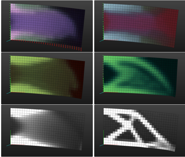
Fig. 8. Resulting material property distributions when running our topology optimization algorithm in the orthotropic ( top left ), cubic ( top right ), isotropic ( middle left ) and an analytically defined gamut E \geq \rho^3 E_0 ( middle right ), with the material property space dimensions ranging from five to two. We compare our algorithm with the standard SIMP method with power index p = 1 ( bottom left ) and p = 3 ( bottom right ). For these figures, we computed the color of each cell by mapping every base vector of the normalized parameter space to a color range and linearly interpolating the colors associated to each of the parameters. In this example, the left side of the cantilever is fixed while a discretized, linearly varying, distributed force is applied to the bottom side (see red arrows in the top left picture).
