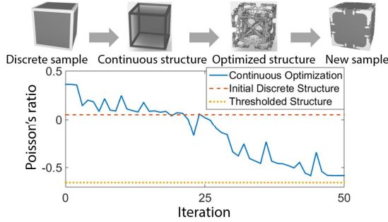
Fig. 5. The continuous sampling step uses topology optimization to expand the gamuts by refining existing structures. A good starting point is necessary for the optimization to find better solutions. We use discrete microstructures near the boundary to initialize topology optimization. At convergence, we threshold the values to obtain a new discrete sample.
