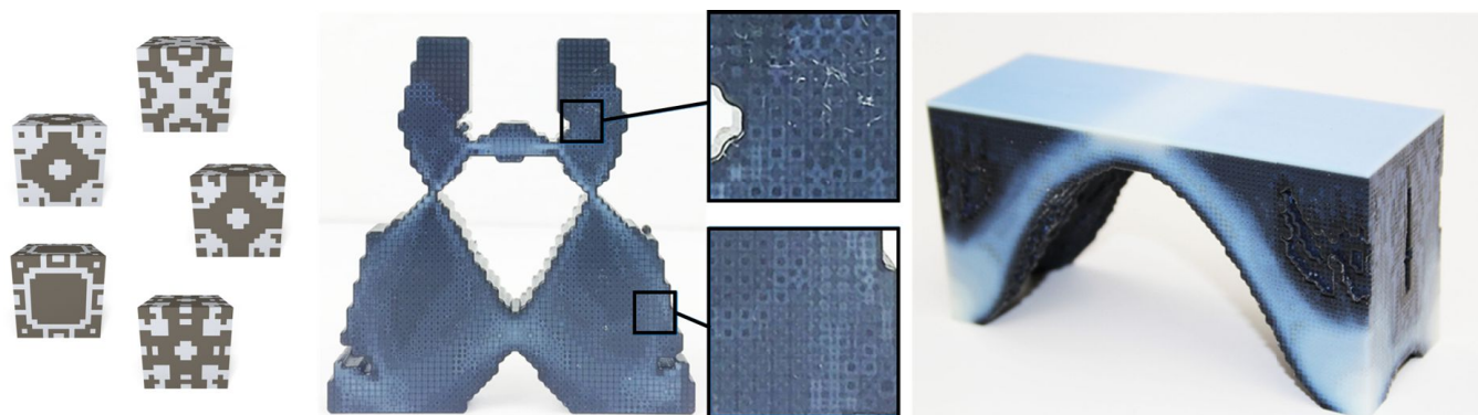
Fig. 1. Our two-scale topology optimization framework allows to optimize continuous material properties mapping to printable microstructures ( left ) to fabricate high-resolution functional objects ( middle ) and minimum compliant structures ( right ).
