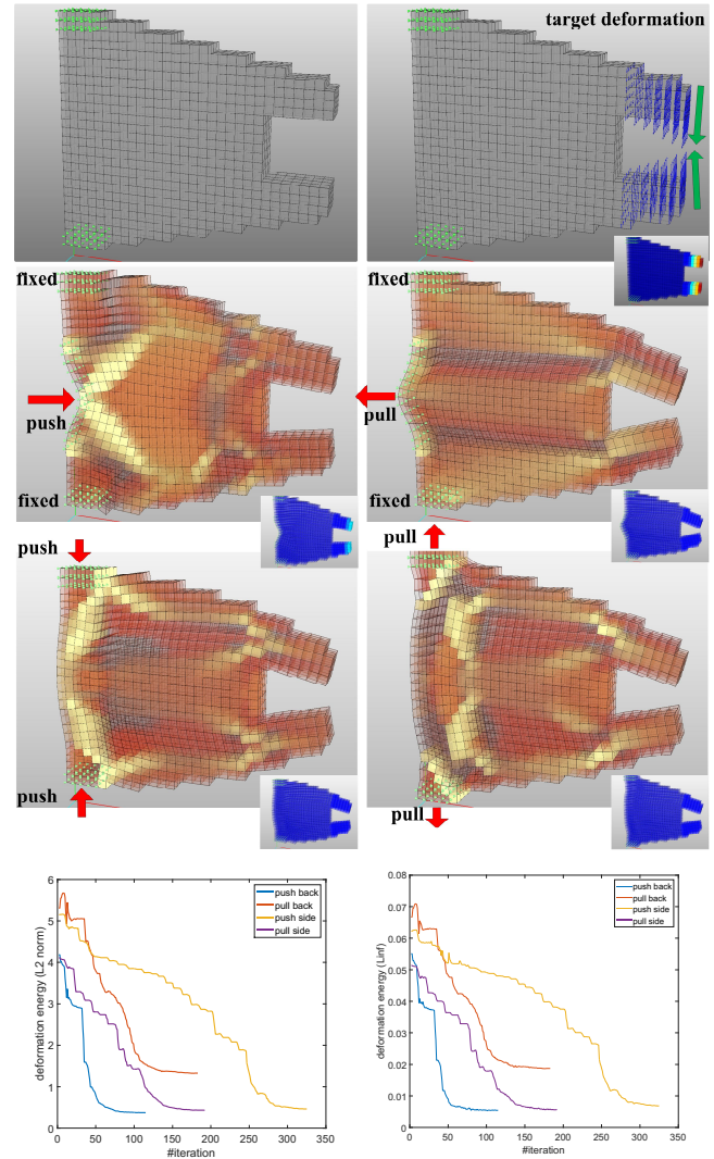
Fig. 13. Designing functional grippers. The top row shows the initial shape of the gripper (left), and the target deformation for the tip (right). The green dots correspond to the fixed vertices while the blue arrows correspond to the target displacements. The two middle rows correspond to the optimized results obtained for the specified boundary conditions. The inset pictures color-code the initial and final deformation error for the different examples. The convergence plots in the bottom row depict the change in the sum of the deformation errors corresponding to all the cells (left) and the value of the maximal cell error contribution (right) as the optimization progresses.
