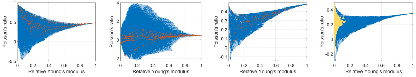
Fig. 6. Gamuts computed with our discrete-continuous sampling scheme for 2D cubic structures ( left ), 2D orthotropic structures ( second from left ), 3D cubic structures ( second from right ) and 3D cubic structures with 0.35 as Poisson's ratio ( right ). The plots show the results for the projection of the gamuts on the plane defined by the macroscale Young's modulus along the x axis (normalized by the Young's modulus of the stiffest base material) and the Poisson's ratio corresponding to a contraction along the y-direction when the material is stretched along the x-direction. The blue dots correspond to the generated samples, the orange dots correspond to the microstructures from Schumacher et al. [2015] and the yellow dots correspond to the microstructures from Panetta et al. [2015].
