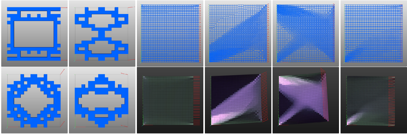
Fig. 18. Optimizing the orthotropic material parameters of a single cell ( left ) and a 32 \times 32 lattice of cells ( right ) subject to directional forces. The vertices on the left side of the layout are fixed while forces are applied on the right vertices as depicted by the red arrows. Our simple but effective tiling algorithm allows to nicely transition between microstructures of smoothly material properties ( right, top ).
