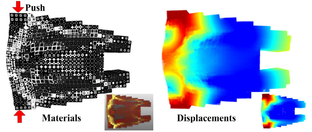
Fig. 16. Comparison of a simulated gripper with homogenized material properties ( inset picture, left ) to the one using full microstructures ( main picture, left ). The figures on the right show the vector field of vertex displacement of the two models. The blue-to-red colors represent the magnitudes of the displacements.
