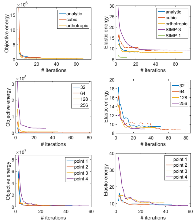
Fig. 9. Convergence tests. Variation of the objective energy ( left ) and the elastic energy ( right ) of a beam being optimized for minimum compliance as the optimization progresses. The convergence plots correspond to the beam of Figure 8 when optimized using different material spaces ( top ), different resolutions for the beam lattice ( middle ) when using cubic microstructures, and different initial material properties for the cubic microstructures ( bottom ).
