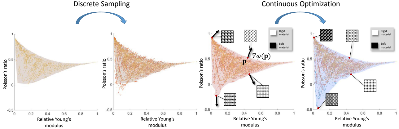
Fig. 4. One cycle of computing the microstructure gamut. Given a set of samples, we compute a signed distance function approximating the material gamut ( left ) and randomly perturb microstructures lying near the boundary to provide new seeds to the continuous algorithm ( middle left ). We then update the distance field and use the gradient of the signed distance function at the the boundary to define new target material points ( middle right ). These target material points are used in a continuous optimization that generates new samples ( right ).
