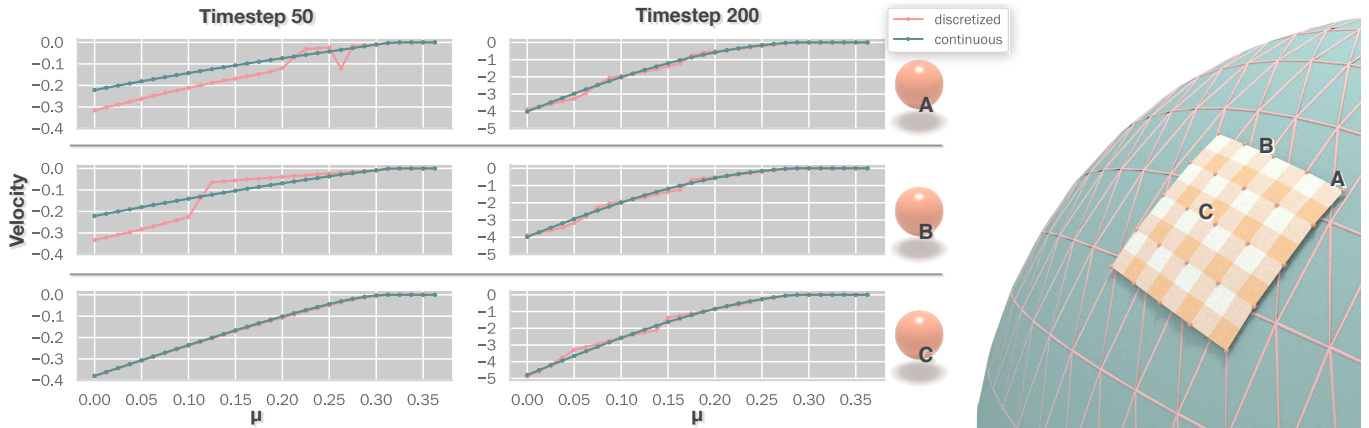
Fig. 2. We simulate a piece of cloth sliding on a rigid sphere (right) to study the discontinuities and non-smoothness from contact conditions and surface geometry (Sec. 5.1). The two columns of plots show the velocities of three contact nodes at the 50-th and 200-th time steps. The “discretized” and “continuous” labels indicate whether these velocities are computed with a triangulated sphere (visualized as pink triangles on the spherical surface) or a smooth sphere (visualized as green sphere surface).
