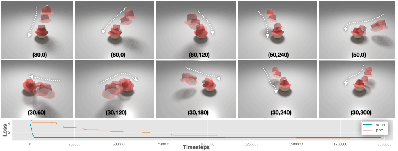
Fig. 12. Hat Controller. We train a closed-loop controller for the advanced “Hat” task (Sec. 6.5) which aims to move the hat from different initial positions (sampled from a fixed-radius hemisphere) onto the head. Top two rows: We visualize the control trajectories of the hat in ten initial positions denoted by their elevation and azimuth angle at the bottom of each subfigure. Bottom: The loss vs. time step curve for our gradient-based optimization and PPO.
