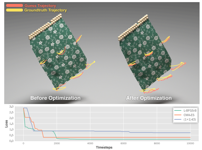
Fig. 11. Flag . A real-to-sim example that reconstructs a digital flapping flag (540 vertices, 1026 triangles, h = 1/120s , 100 time steps) based on motion data captured from real-world experiments. Top: We plot the trajectories of 6 nodes on the cloth from the ground-truth motion (yellow curves) and the simulation results with guesses on the material and wind parameters before optimization (orange curves, left) and after optimization (orange curves, right). Bottom: The loss vs. time step curves for all methods.
