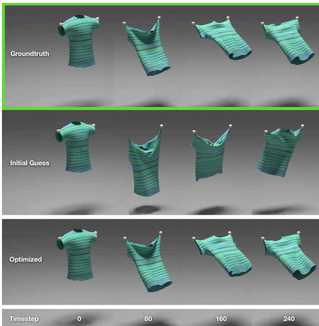
Fig. 7. T-shirt (4278 DoFs, h = 1/90s , 250 time steps). Estimating the cloth material and wind parameters based on a given synthetic motion sequence of the T-shirt. From left to right we show the simulated T-shirt at 0, 80, 160, and 240 time steps. Top: the ground-truth motion sequence; Middle: simulation with the initial guess on the cloth and wind parameters; Bottom: simulation after optimization with L-BFGS-B.
