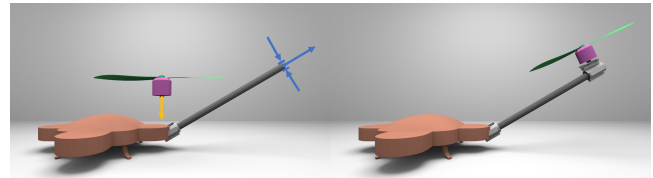
Figure 3: Example of composition. Left: parts with highlighted patches (circular patch with an annotated main axis and a diameter in blue and flat patch with an annotated normal in orange). Right: composed design.
