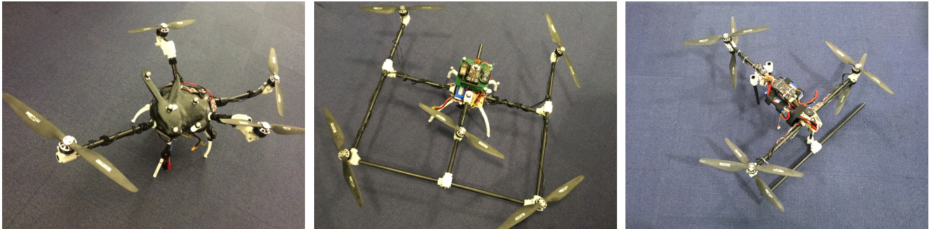
Figure 1: We provide an interactive system for users to design, optimize and fabricate multicopters. We explore the design space to allow multicopter design with free-form geometry and nonstandard motor positions and directions. Based on user-specified metrics, our system optimizes the copter geometry and suggests a valid controller. Left: a multicopter example with free-form geometry, various motor heights and different propeller sizes. Middle: a pentacopter with optimized motor positions and orientations, allowing 30% increase in payload. Right: a classic hexacopter with three pairs of coaxial propellers.
