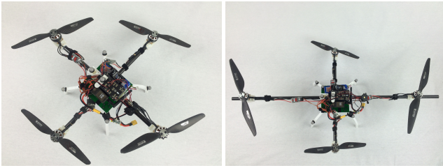
Figure 9: Optimizing a quadcopter with flight time metric and geometry constraints. Left: a standard quadcopter. Right: optimized rectangular quadcopter.
