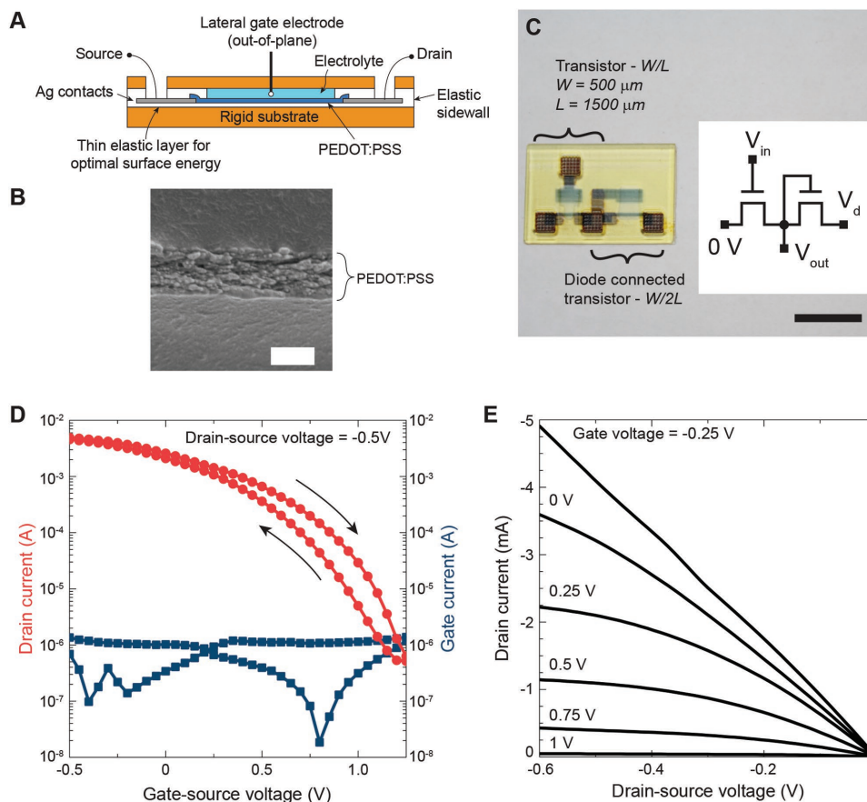
Figure 3. Printed depletion mode p-type PEDOT:PSS transistors. a) A cross-sectional schematic of the transistor is shown. b) Scanning electron microscope image of PEDOT:PSS layer between elastic polymer layers. Scale bar is 1 \mu\text{m} . c) Photograph of a transistor amplifier with a diode connected load. Transistor width, W = 500 \mu\text{m} and length, L = 1500 \mu\text{m} . The diode connected transistor has a length 2L = 3000 \mu\text{m} . Scale bar is 10 mm. (Performance characteristics of diode connected loads, and the input-output characteristics of the amplifier are in Figure S7d and Figure S7e respectively.) d) Drain current and gate current of a transistor as a function of the gate-source voltage. Transistor has width, W = 500 \mu\text{m} and length, L = 1500 \mu\text{m} . e) Transistor I - V curves showing drain current as a function of drain voltage, for gate voltage between -0.25 \text{ V} and 1 \text{ V} , in steps of 0.25 \text{ V} . (Plots of the transconductance and sub-threshold swing, response time and characteristics of multiple devices printed in separate runs are in Figure S7.)
